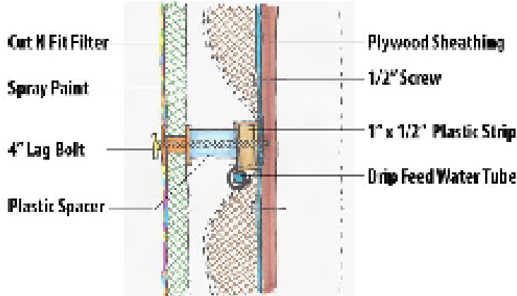
Connection Detail 01
